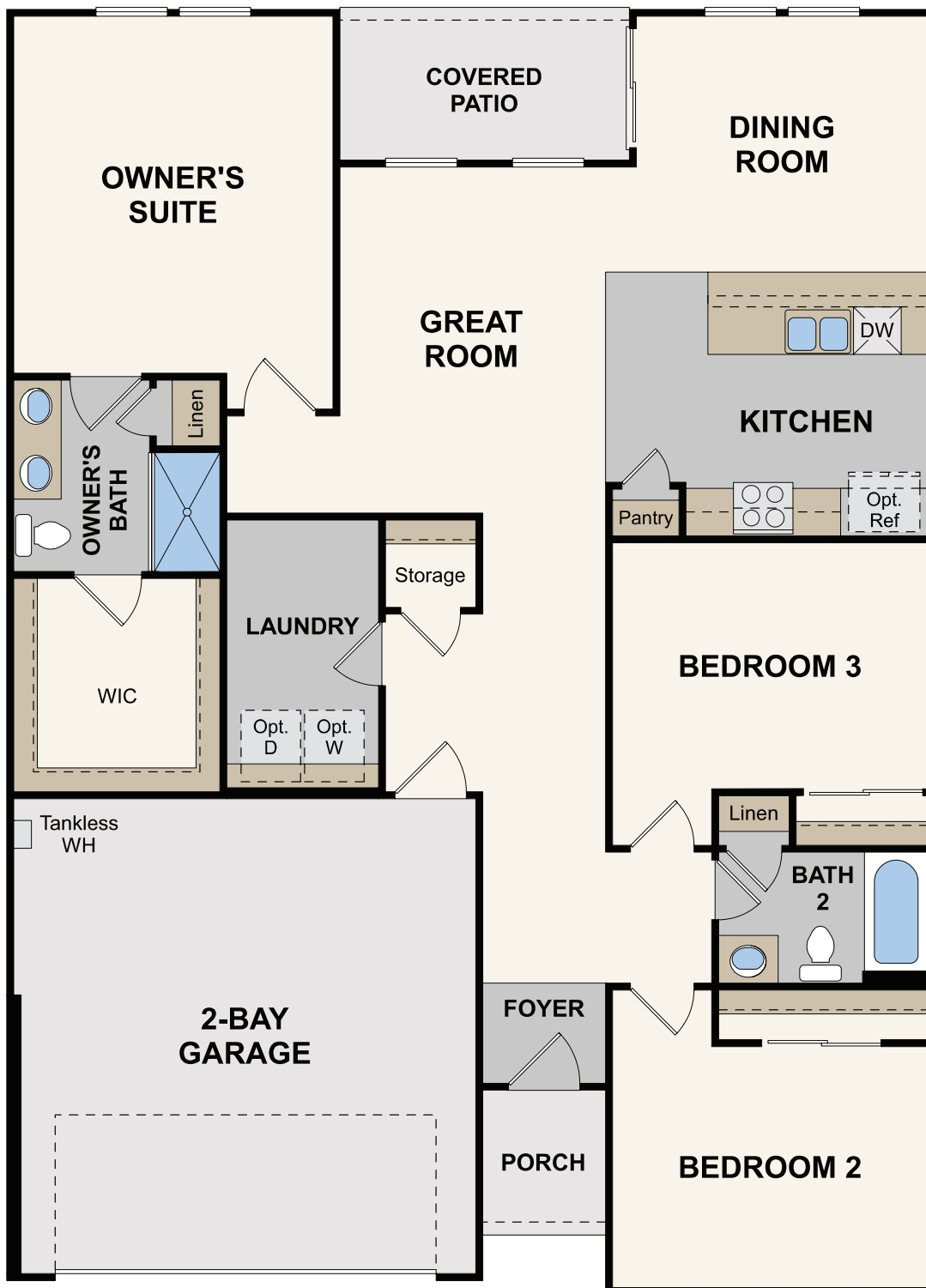
FLOOR PLAN
